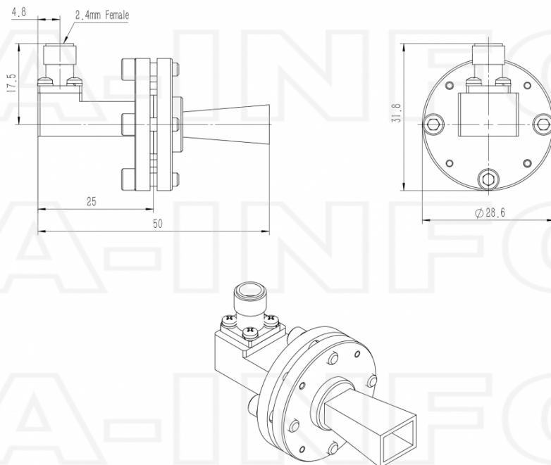
2.4mm-Female Output (P/N: LB-19-10-C-2.4F)
